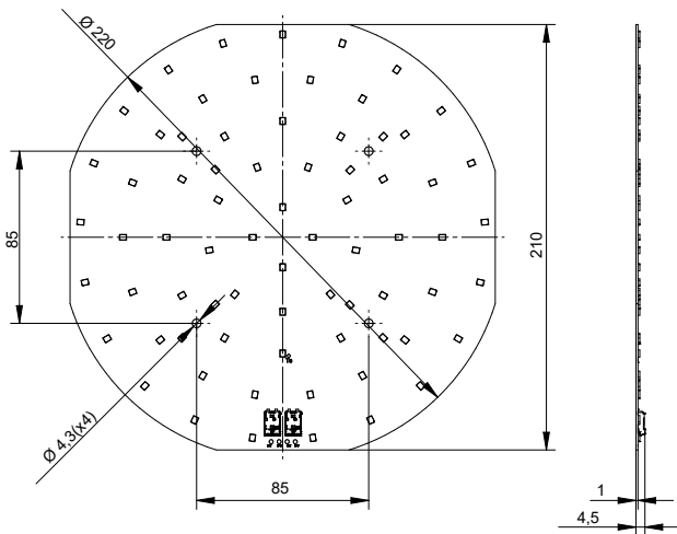
RdLED 220mm
