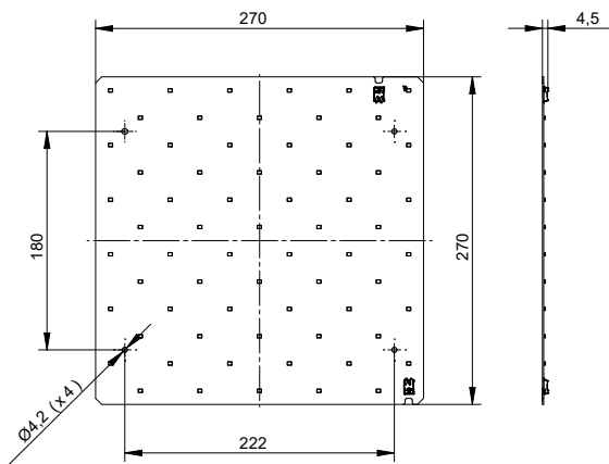
RecLED 270x270mm
