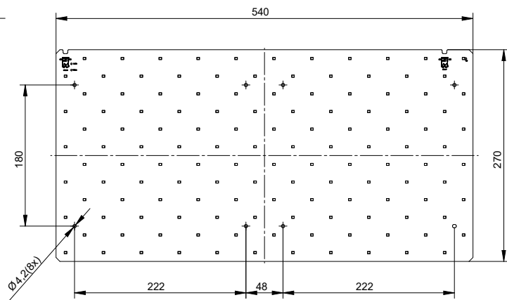
RecLED 540x270mm
