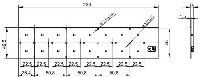
RecLED 224x50mm 2x8
