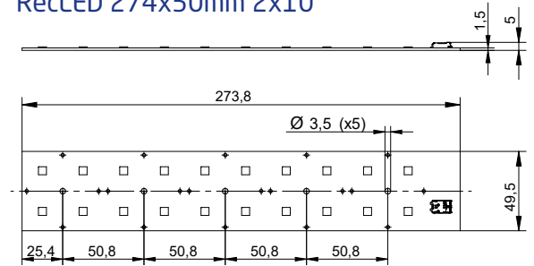
RecLED 274x50mm 2x10
