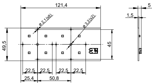
RecLED 122x50mm 2x4
