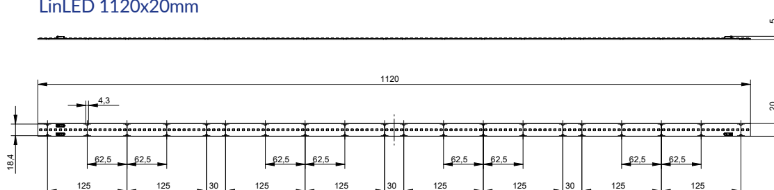
LinLED 1120x20mm
