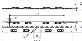
LinLED 140x24mm 2x500lm 2x4C 42V
