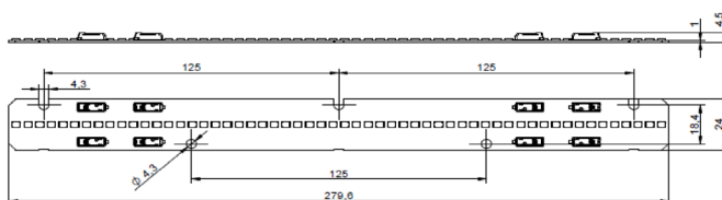
LinLED 280x24mm 2x1000lm 2x4C 42V
