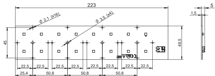
RecLED 224x50mm 2x8
